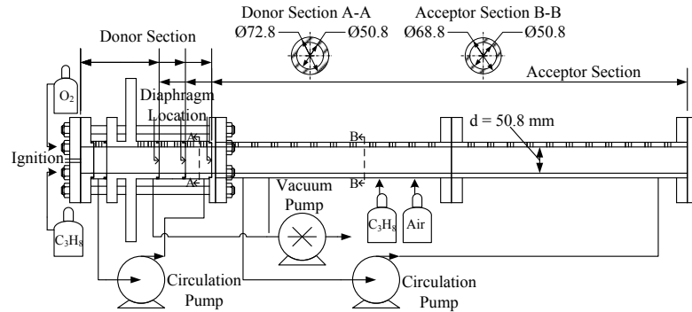
Fig. 1. Experimental facility
